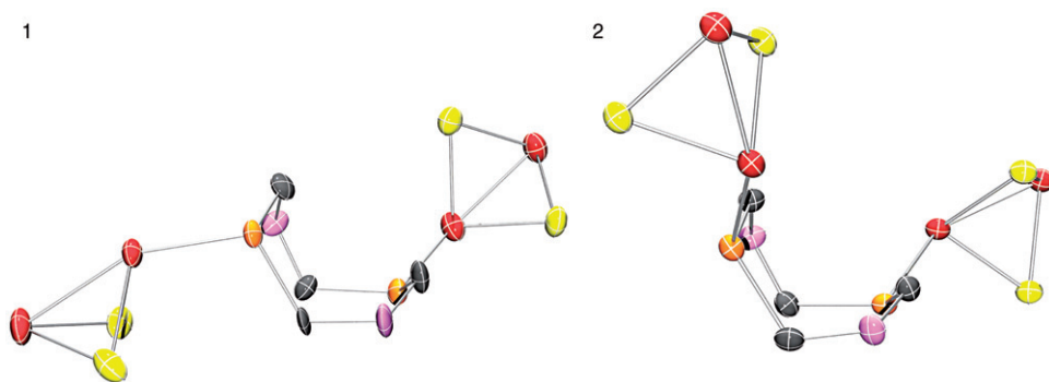
Figure 3. Structural details of 1 and 2 highlighting the coordination mode of the bridging P_2^R N_2^{Ph} unit with respect to the Fe_2S_2 cores.
