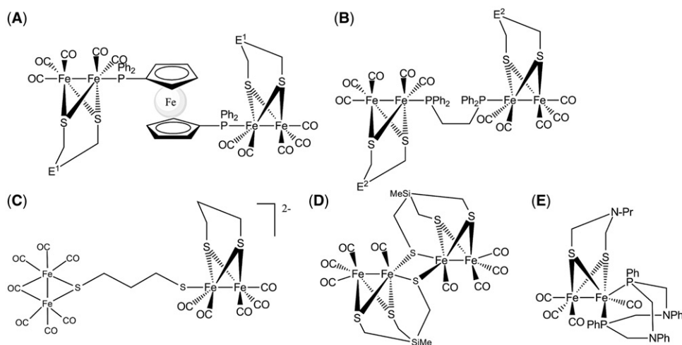
Figure 1. Overview of tetranuclear iron complexes A–D and the dinuclear complex E . (A) Ferrocenylbisphosphine (dppf) bridged diiron clusters, where E^1 = \text{CH}_2 [31] or O [32]. (B) Diphenylphosphinoethane (dppe) bridged \text{Fe}_2\text{S}_2 clusters, where E^2 = \text{CH}_2 or \text{N}^i\text{Pr} [30] or \text{CH-O-benzyl} [33]. (C) Two \text{Fe}_2 units bridged by a propyldithiolate (pdt) moiety [35]. (D) Two \text{Fe}_2\text{S}_3 cores are connected via two \kappa^2 sulfur units [34]. (E) \text{P}_2\text{N}_2^{\text{Ph}} acting as a bidentate ligand toward the same iron center [28].
